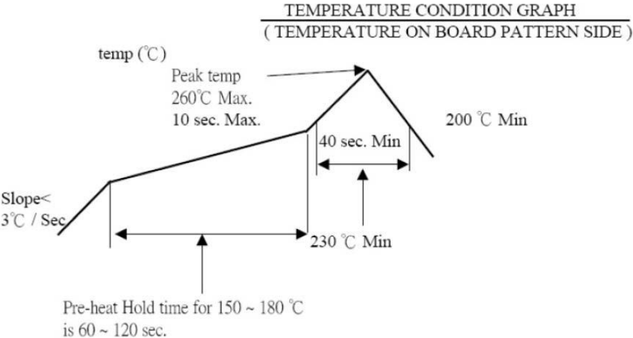
Figure 1 Recommended temperature profile of infrared reflow. (图 1 为红外回流焊推荐温度曲线图)
