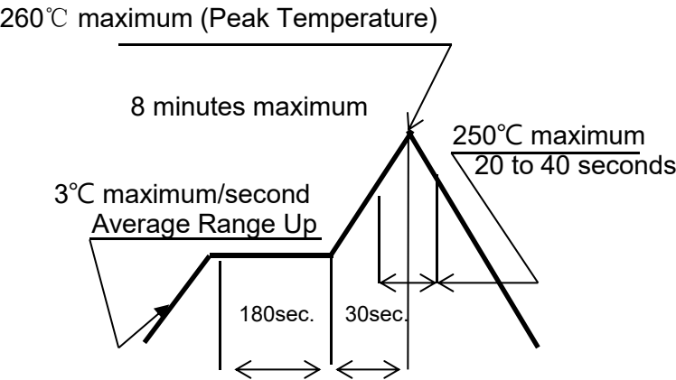
(Preheat Temperature预热温度: 150~200°C Maximum.) Temperature Condition Graph.温度状态图 (Temperature on Board Pattern Side )
